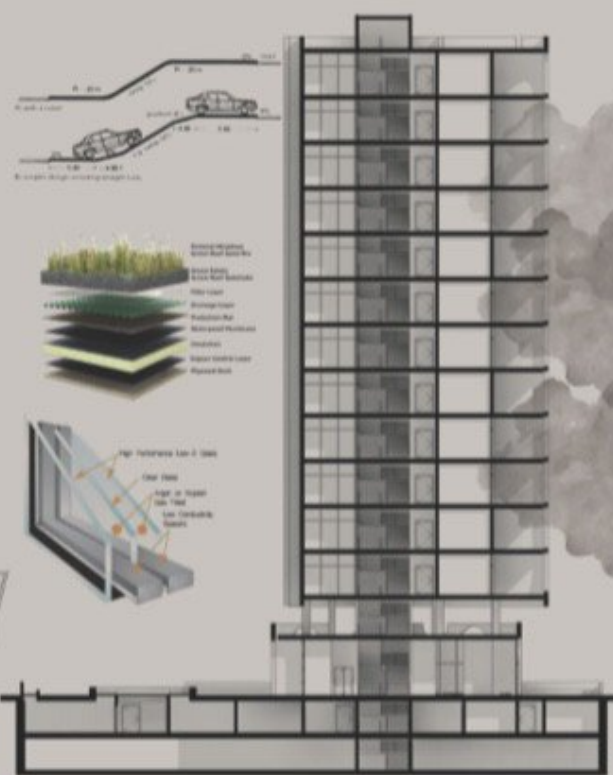
SECTION AA 1/200
